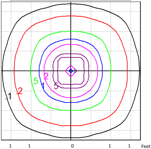
HDBS 35W FOOT CANDLE ISOLINE
