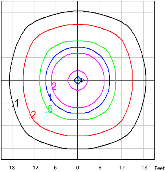
HDBS 25W FOOT CANDLE ISOLINE
